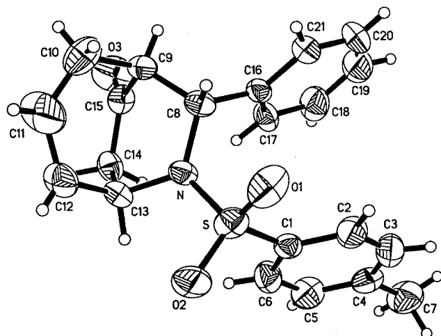
Figure 3. The crystal structure of exo-7a
