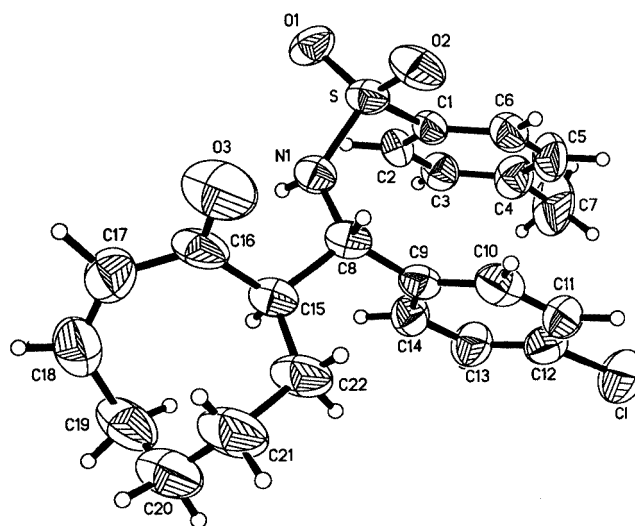
Figure 4. The crystal structure of 9b
