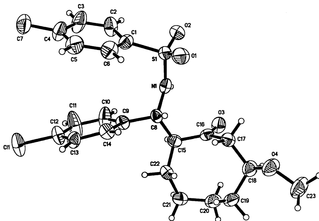
Figure 5. The crystal structure of 10c
