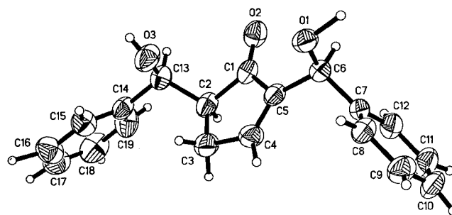
Figure 1. The crystal structure of syn - 3b
