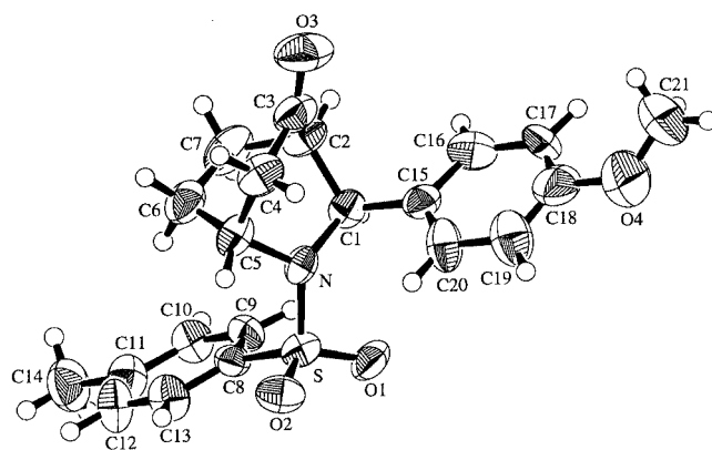
Figure 2. The crystal structure of exo-5d
