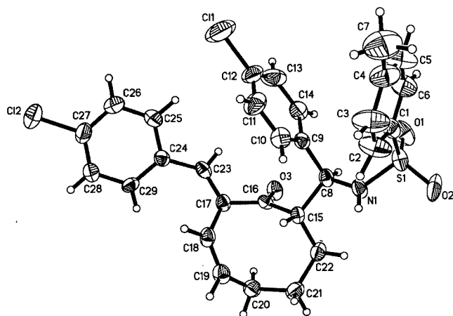
Figure 6. The crystal structure of 12b
